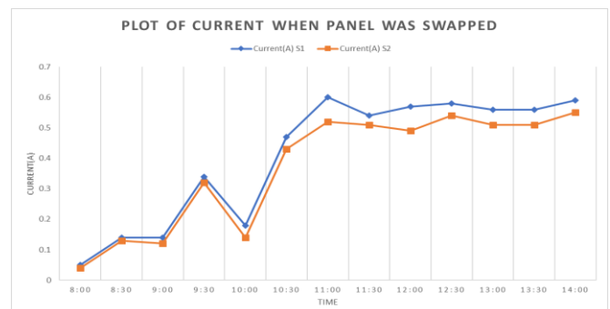
Fig. 12. Plot of current of S1 and S2. (Swapped)
